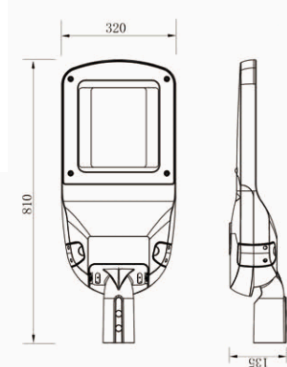
180W AXSL01
