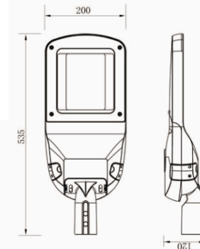
50W AXSL01
