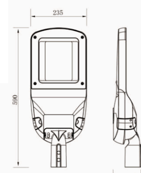
80W AXSL01
