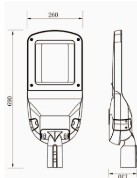
120W AXSL01
